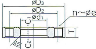
⓪ FLANGES
